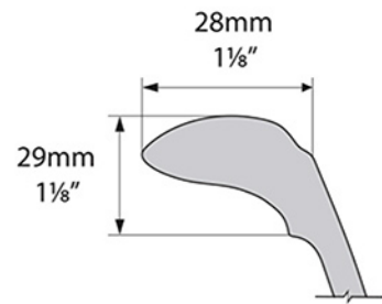
Rim detail
